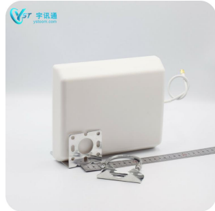
YP-2400/2700-14D-SMA
