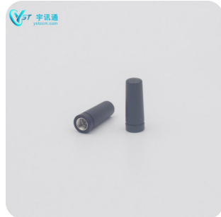
YW-1200/1575-2D-SMA
