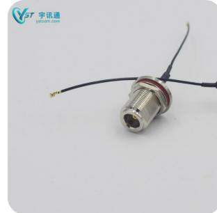
YC-Nf/UFL-1.37/10CM-01
