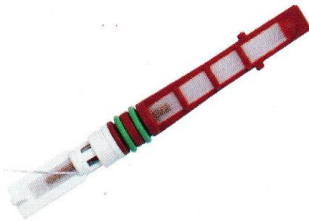
YX99510 节流阀
