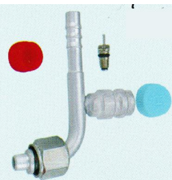
优质接头带134a阀 High-quality adapter with 134a valve 3/8 O 90° 带134a阀 3/8 O 90° with 134a valve
