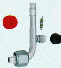
优质接头带R12阀 High-quality adapter with R12 valve 3/8 O 90° 带R12阀 3/8 O 90° with R12 valve
