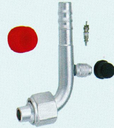
优质接头带R12阀 High-quality adapter with R12 valve 1/2 O 90° 带R12阀 1/2 O 90° with R12 valve
