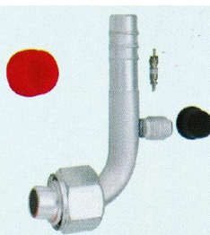
优质接头带R12阀 High-quality adapter with R12 valve 5/8 O 90° 带R12阀 5/8 O 90° with R12 valve
