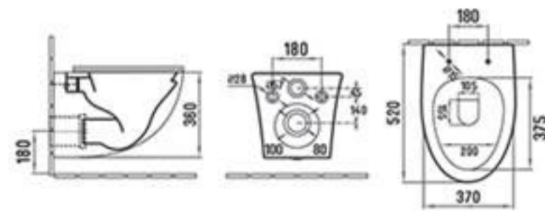
B2352 Wall-hung toilet Size: 520x370x360mm P-trap: 180mm Rouging-in
