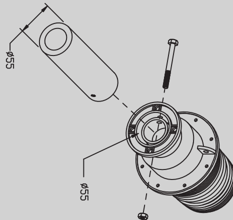
Fit 55mm diameter hollow-rod
