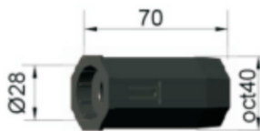
Calotta oct40 per cuscinetto Od28 Kapsel oct40 für Kugellager Od28 Plastic cap oct40 with bearing housing dia.28mm 塑料尾插, oct40,配OD28轴承
