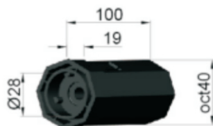
Calotta oct40 per cuscinetto Od28 Kapsel oct40 für Kugellager Od28 Plastic cap oct40 with bearing housing dia.28mm 塑料尾插, oct40,配OD28轴承
