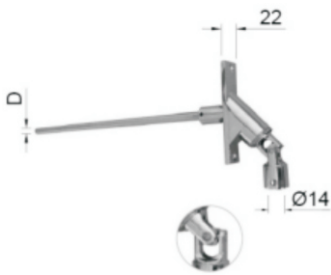
Snodo 90° Kreuzgelenk 90° Cardan Joints 90° 90° 铆接款万向节
