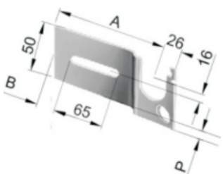
Mensole per supporti Mantova DX Bracket for Mantova supports, right 冲压轴承支架，右
