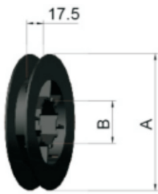
Puleggia in plastica per calotte art 407.101.284 Kunststoff gurtscheibe für art.407.101.284 Plastic pulley for cap 407.101.284 塑料轮盘, 可配407.101.284配套使用
