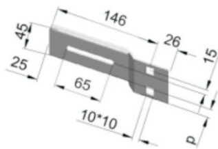
Mensola per supporti TORINO con fori ■10 Bracket for Torino support with two holes ■10 10mm 双方孔支架
