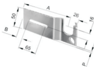
Mensole per supporti Mantova DX Bracket for Mantova supports, right 冲压轴承支架, 右
