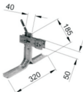
Kit:Supporti"NAPOU"con mensole Kit:"NAPOU"supports with brackets "NAPOLI"支架成套
