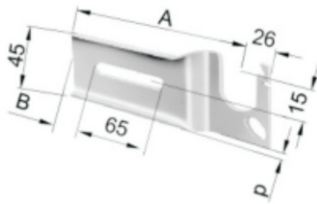
Mensole per supporti TORINO SINISTRE Bracket for Torino supports right(reverse) 冲压轴承支架，左
