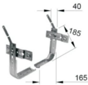
Kit:Supporti"NAPOLI"con mensole Kit:"NAPOLI"supports with brackets "NAPOLI"支架成套
