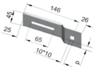
Mensola per supporti TORINO con fori ■10 Bracket for Torino support with two holes ■10 10mm 双方孔支架
