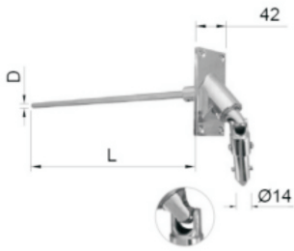
Snodo 90° Kreuzgelenk 90° Cardan Joints 90° ,welded and polished ,90° 焊接款万向节
