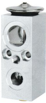
Suit vehicle: SATURN Gas inlet: 10 Liquid inlet: 6 Cas outlet: 12 Liquid outlet: 8 Ton: 0.5-2.5T 1A01121
