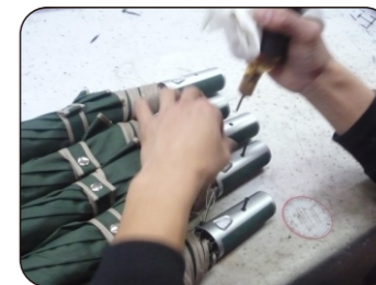
11 装伞头 Fix handle
