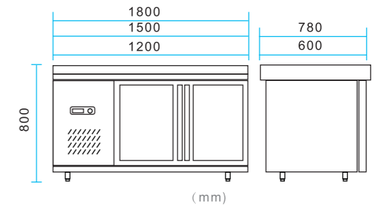
TC0.2L2T / TC0.25L2T / TC0.4L2T
