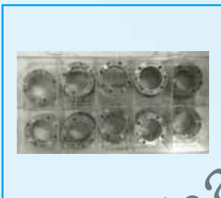
No,122(2) CAT C7C9 Residual Air Gap Adjustment Shims10Kinds x 5pcs=50PCS
