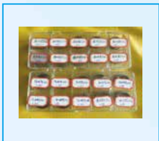
No,109(7) CUMMINS ISG Residual Air Gap Adjustment Shims: 20Kinds x 5pcs=100PCS
