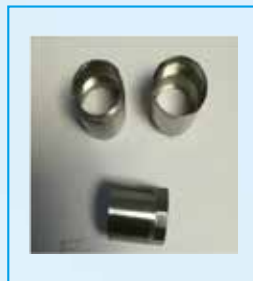
8DT1121A, φ29.3x31.8xM26 For CAT 320D Solenoid Valve
