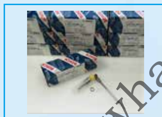
NO.605 BOSCH Genuine overhaul kit F 00Z C99 558
