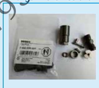
No.587(1) Repair kits F 002 C99 007 for bosch injector 110 series
