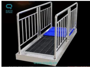
Item: Shoe Polishing Equipment Function: sole clean Material: stainless steel Cleaning Type: Water circulation Switch: auto-induction Water tank capacity: 6L
