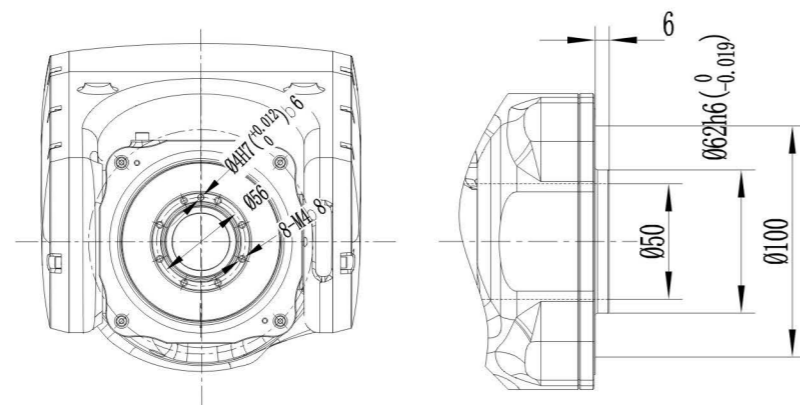
Flange Dimensions
