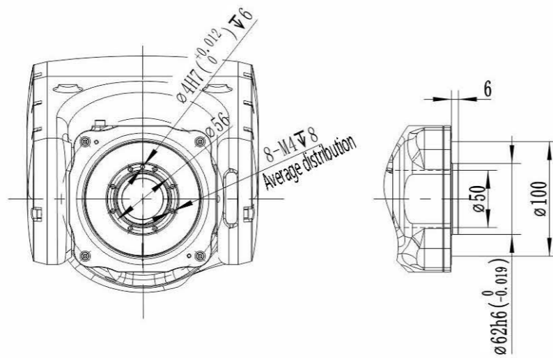
Flange Dimensions
