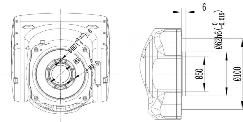
Flange Dimensions
